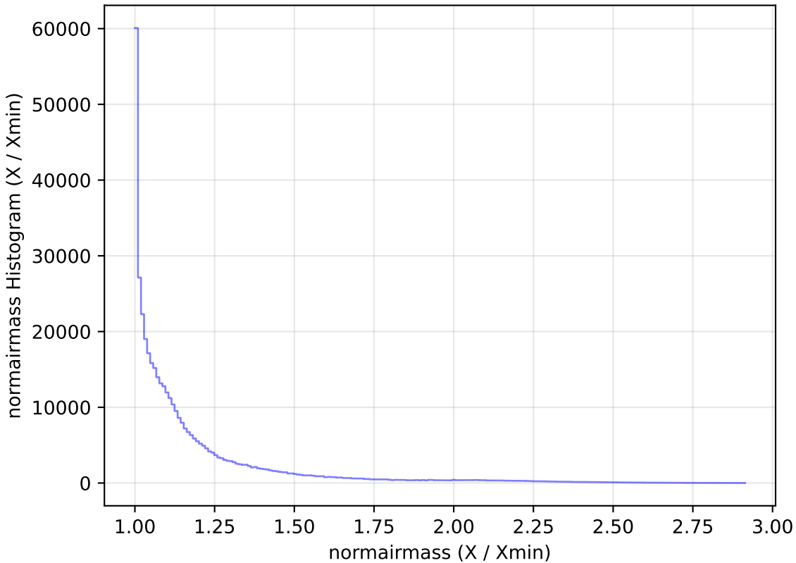
too_elab_r64_d3_gz_v3.4_10yrs WFD z band: normairmass Histogram
