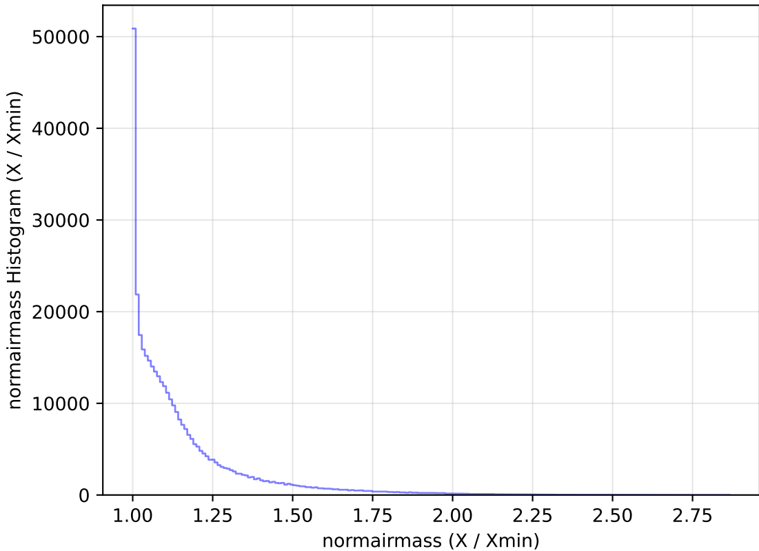
too_elab_r64_d3_gz_v3.4_10yrs WFD y band: normairmass Histogram
