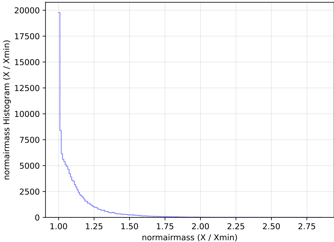
too_elab_r64_d3_gz_v3.4_10yrs WFD u band: normairmass Histogram
