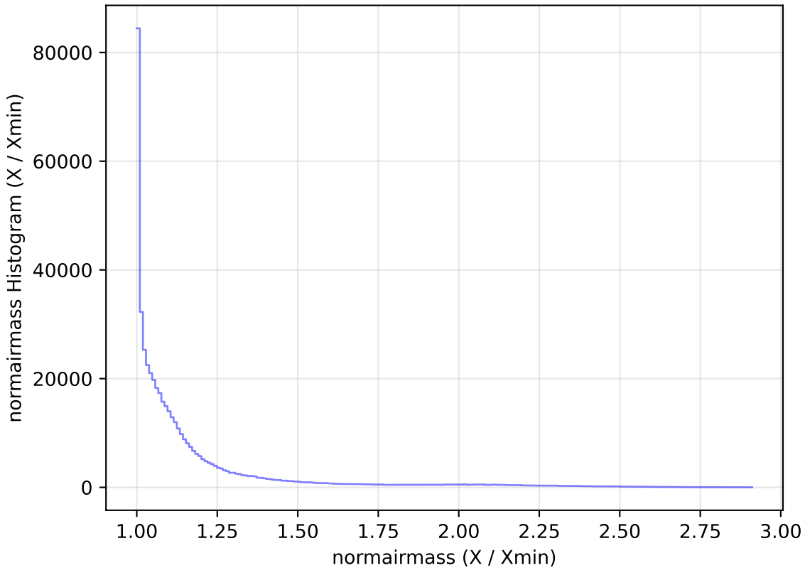
too_elab_r64_d3_gz_v3.4_10yrs WFD i band: normairmass Histogram
