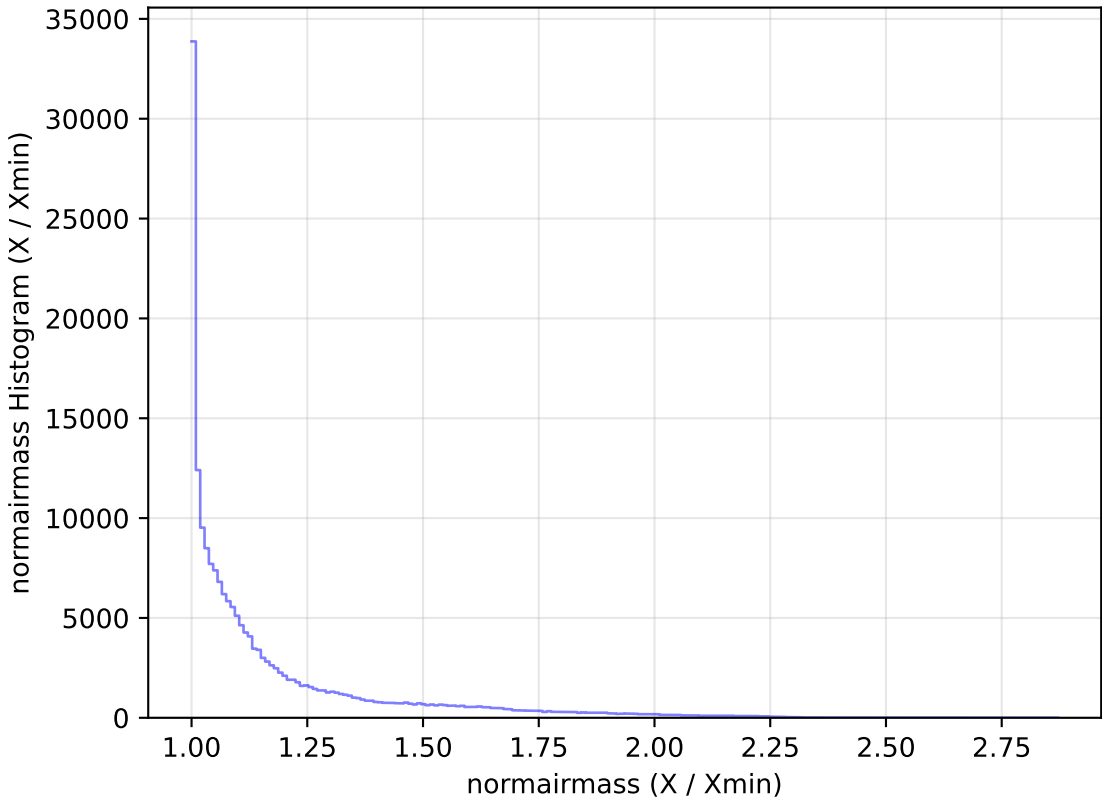
too_elab_r64_d3_gz_v3.4_10yrs WFD g band: normairmass Histogram
