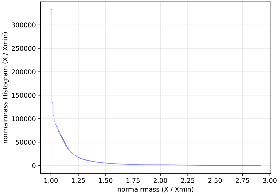
too_elab_r64_d3_gz_v3.4_10yrs WFD all bands: normairmass Histogram
