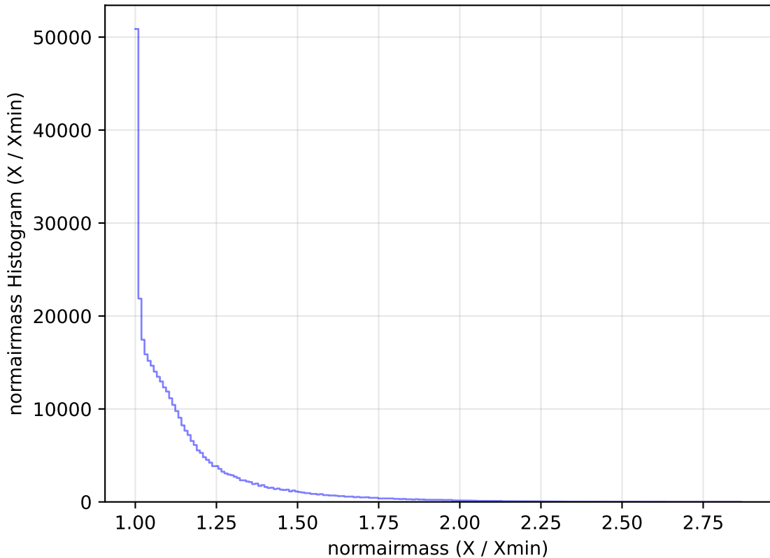
too_elab_r64_d3_gz_v3.4_10yrs All sky y band: normairmass Histogram
