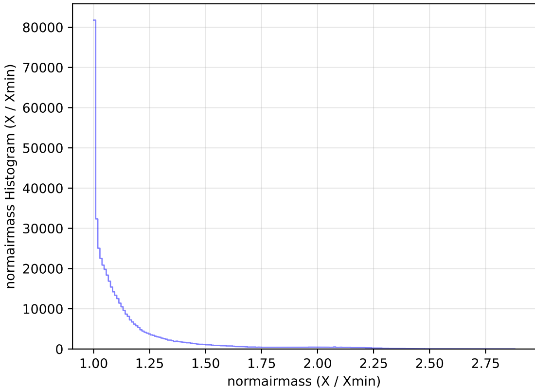
too_elab_r64_d3_gz_v3.4_10yrs All sky r band: normairmass Histogram
