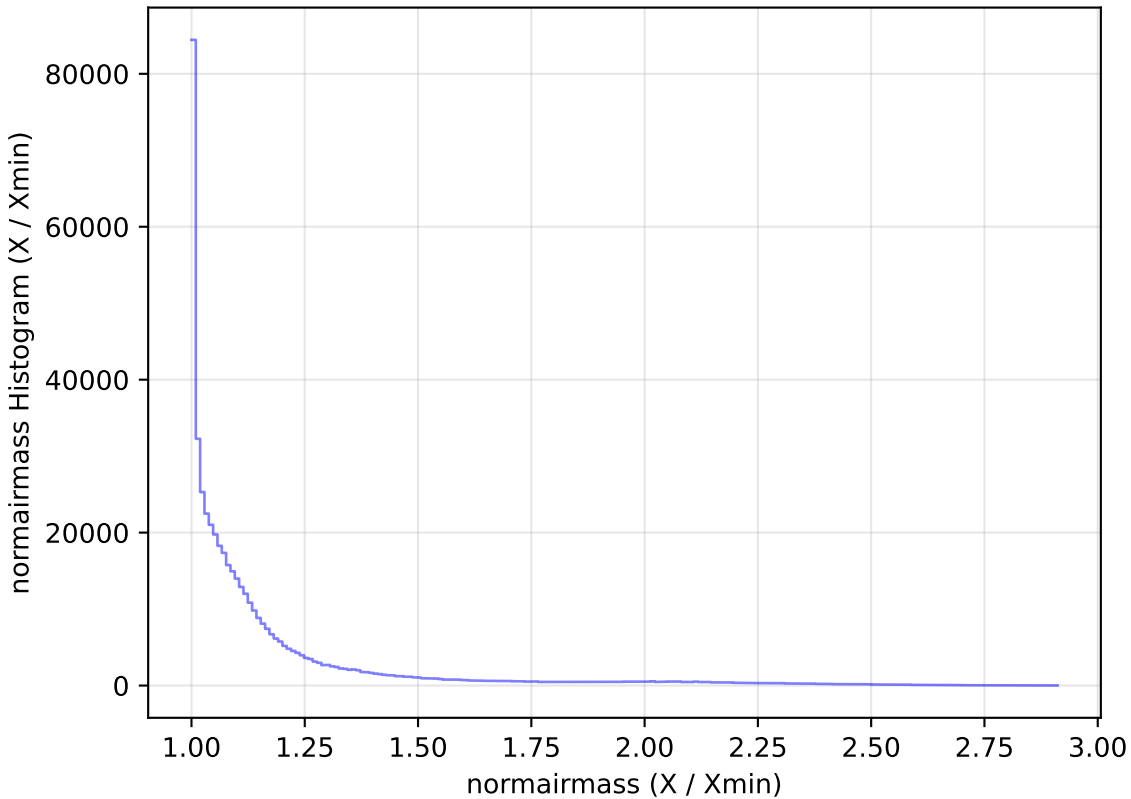
too_elab_r64_d3_gz_v3.4_10yrs All sky i band: normairmass Histogram
