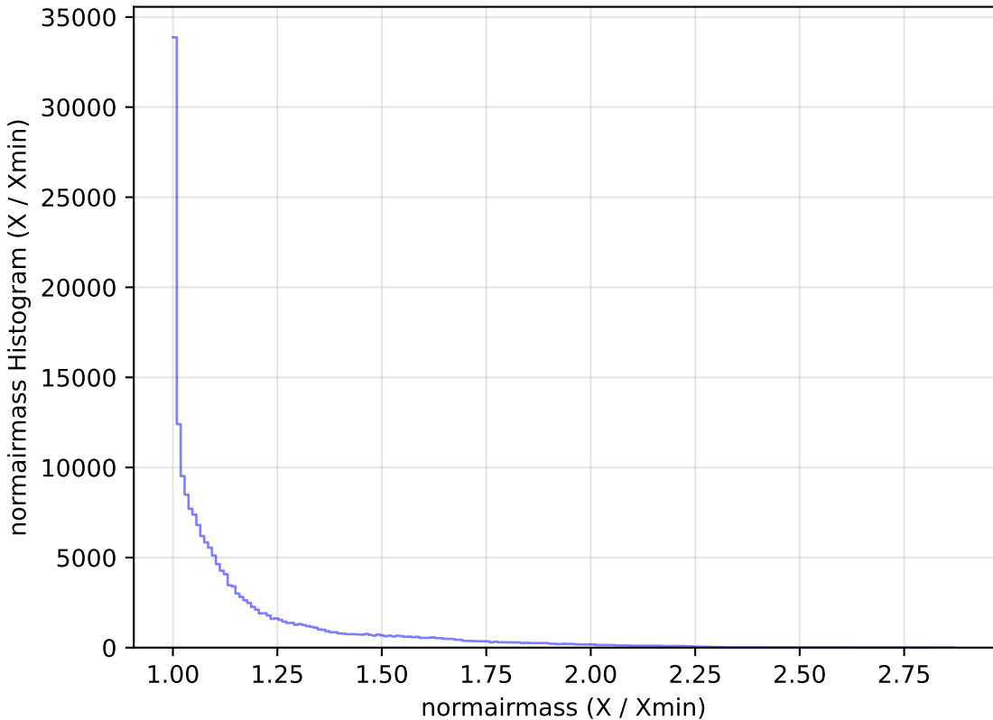
too_elab_r64_d3_gz_v3.4_10yrs All sky g band: normairmass Histogram
