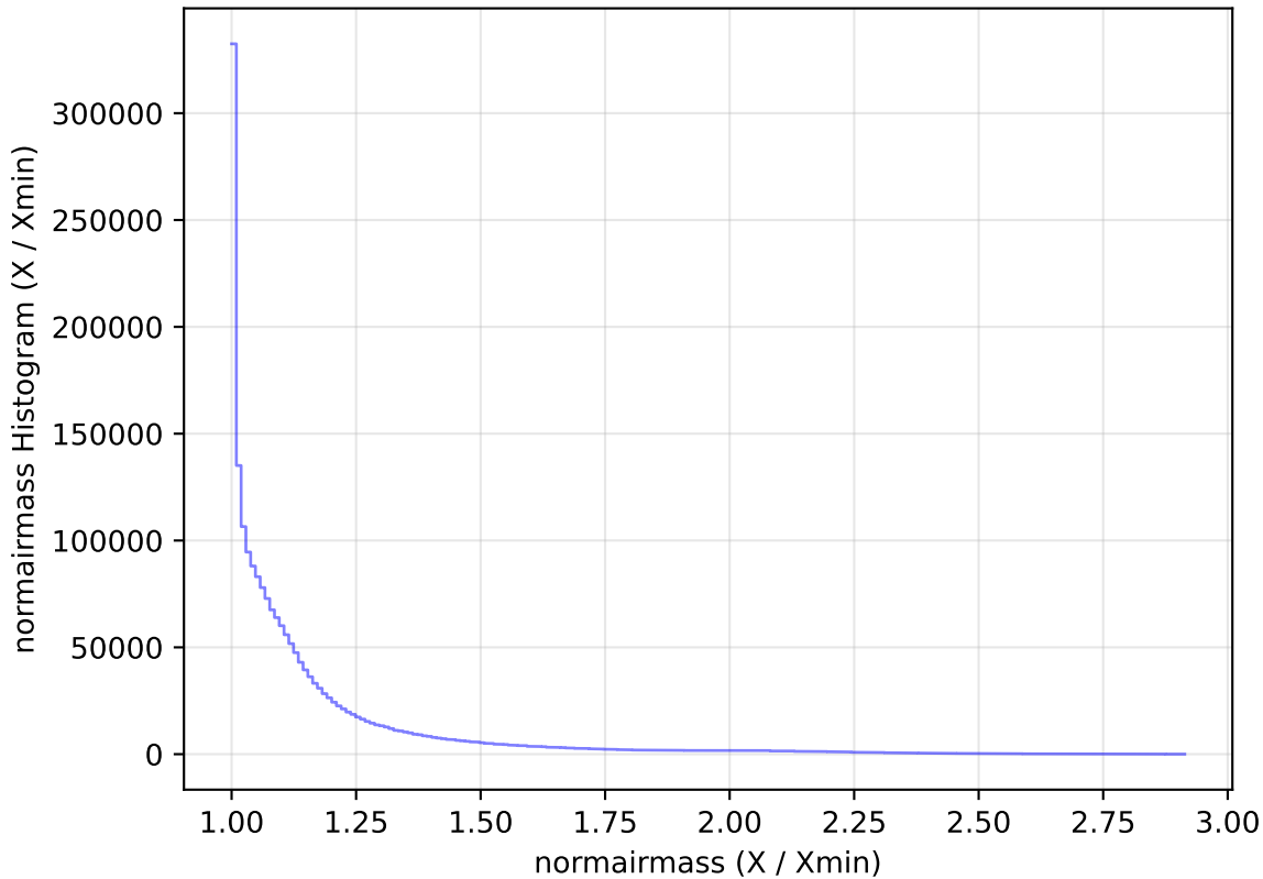
too_elab_r64_d3_gz_v3.4_10yrs All sky all bands: normairmass Histogram
