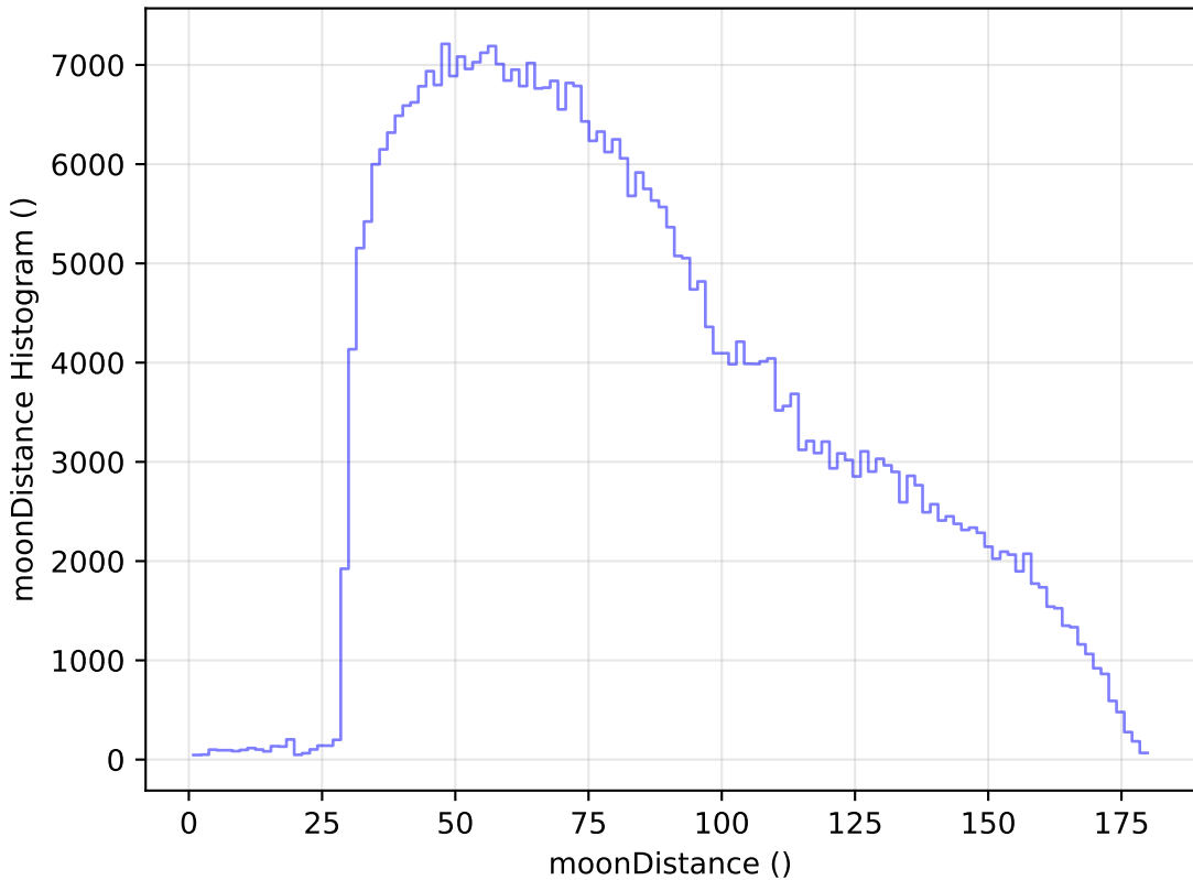
too_elab_r64_d3_gz_v3.4_10yrs WFD z band: moonDistance Histogram
