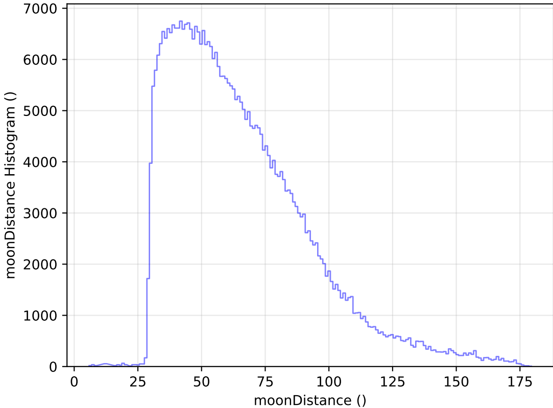
too_elab_r64_d3_gz_v3.4_10yrs WFD y band: moonDistance Histogram
