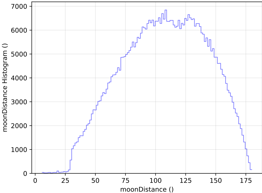
too_elab_r64_d3_gz_v3.4_10yrs WFD r band: moonDistance Histogram
