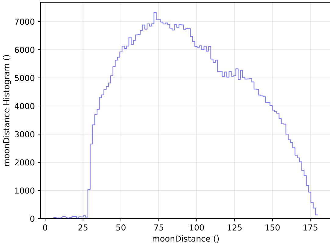
too_elab_r64_d3_gz_v3.4_10yrs WFD i band: moonDistance Histogram
