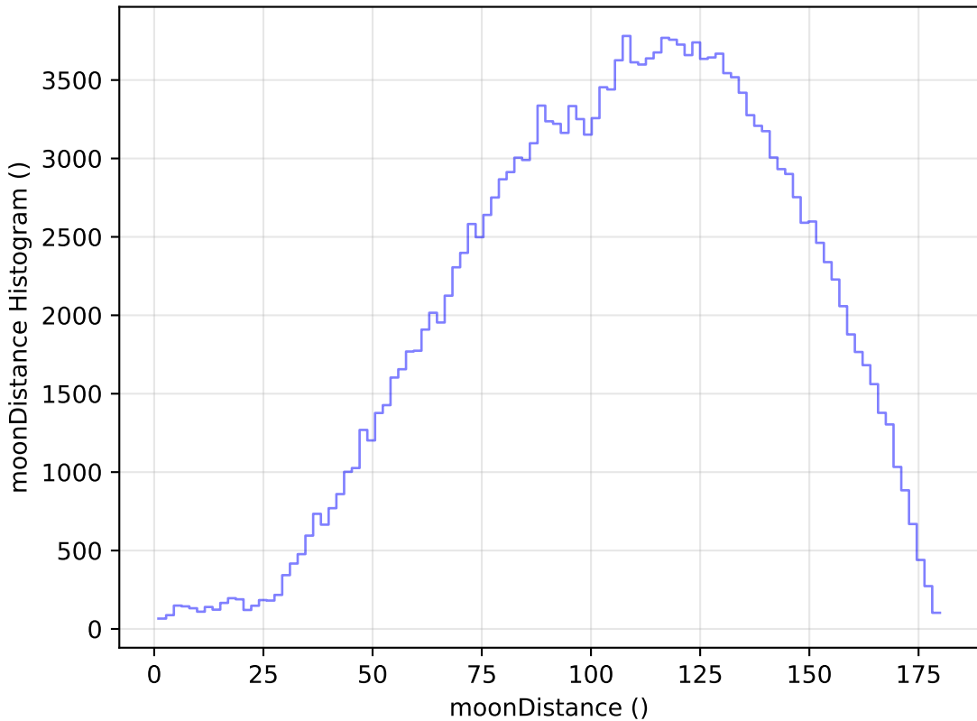
too_elab_r64_d3_gz_v3.4_10yrs WFD g band: moonDistance Histogram
