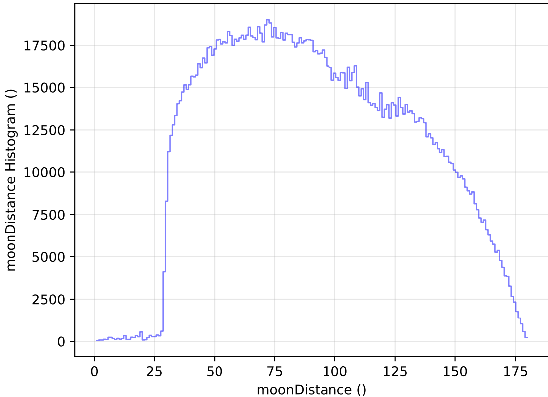
too_elab_r64_d3_gz_v3.4_10yrs WFD all bands: moonDistance Histogram
