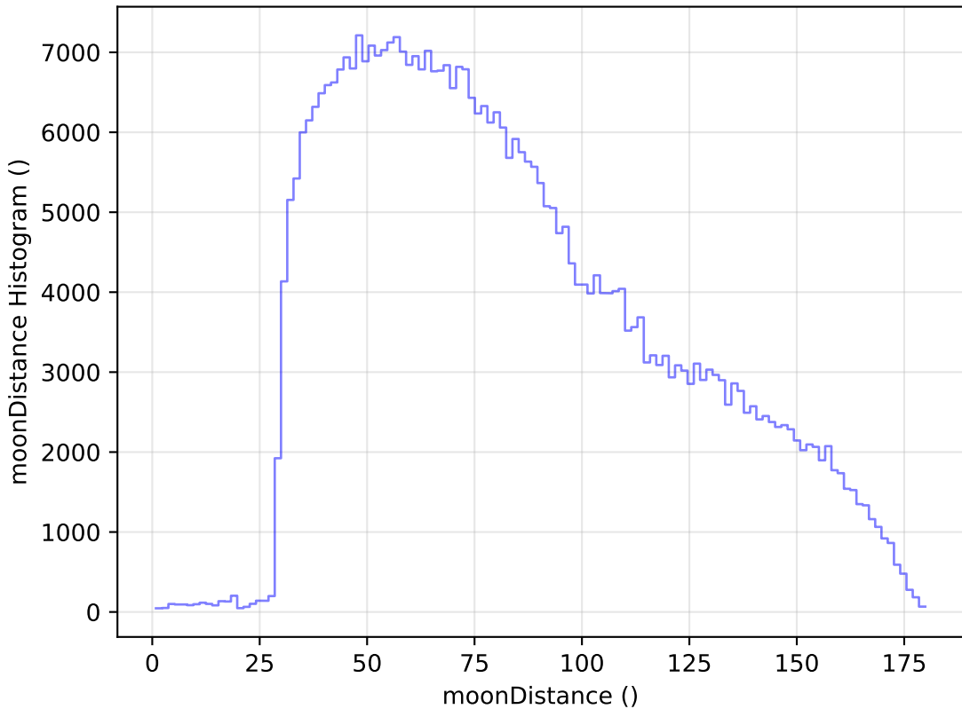
too_elab_r64_d3_gz_v3.4_10yrs All sky z band: moonDistance Histogram
