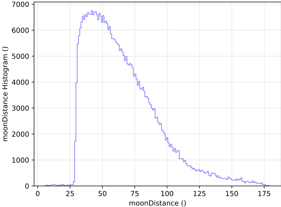
too_elab_r64_d3_gz_v3.4_10yrs All sky y band: moonDistance Histogram
