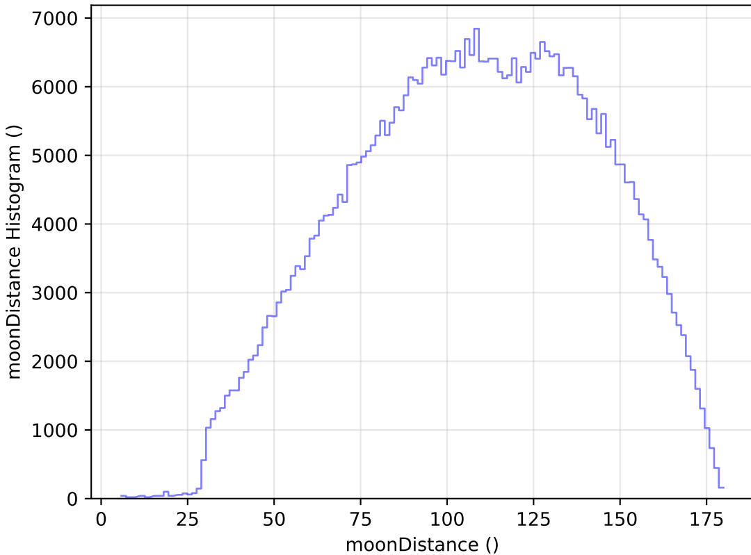
too_elab_r64_d3_gz_v3.4_10yrs All sky r band: moonDistance Histogram
