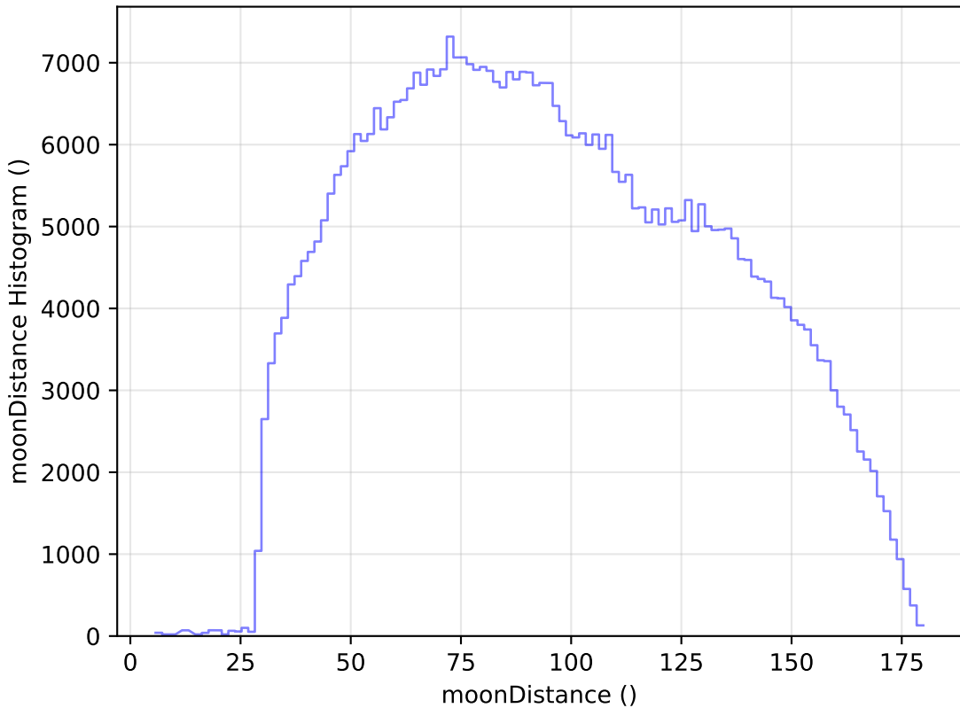
too_elab_r64_d3_gz_v3.4_10yrs All sky i band: moonDistance Histogram
