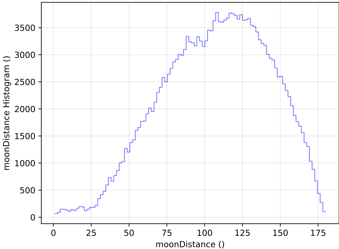
too_elab_r64_d3_gz_v3.4_10yrs All sky g band: moonDistance Histogram
