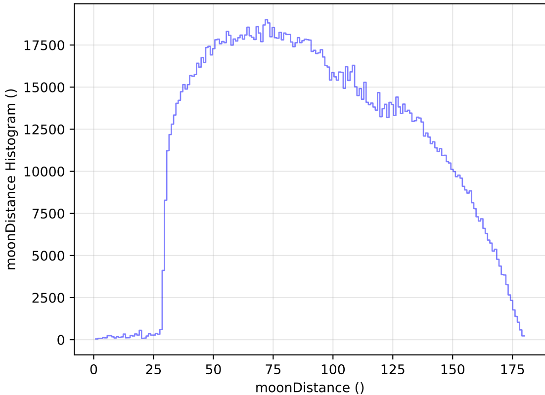
too_elab_r64_d3_gz_v3.4_10yrs All sky all bands: moonDistance Histogram
