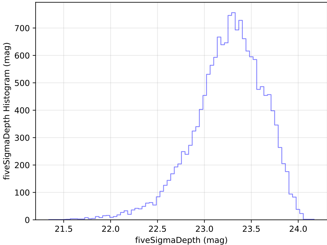
too_elab_r64_d3_gz_v3.4_10yrs Yr 1 u band: fiveSigmaDepth Histogram
