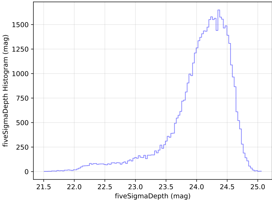
too_elab_r64_d3_gz_v3.4_10yrs Yr 1 r band: fiveSigmaDepth Histogram
