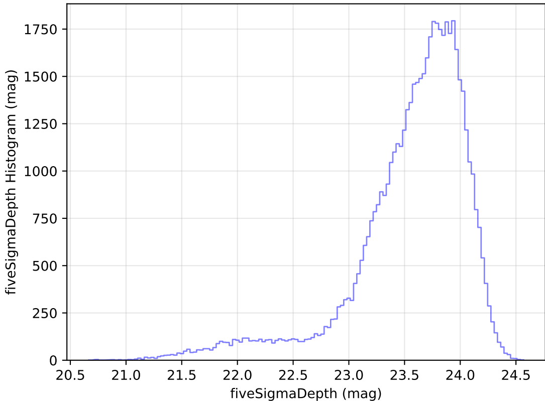
too_elab_r64_d3_gz_v3.4_10yrs Yr 1 i band: fiveSigmaDepth Histogram
