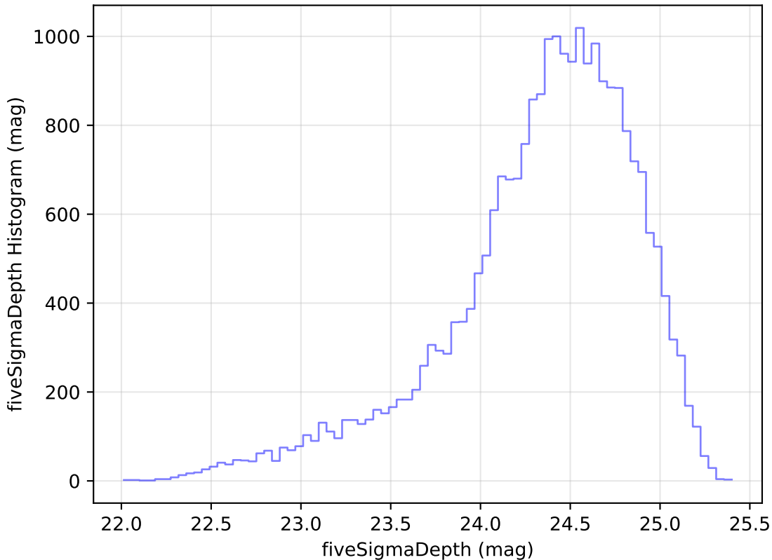
too_elab_r64_d3_gz_v3.4_10yrs Yr 1 g band: fiveSigmaDepth Histogram
