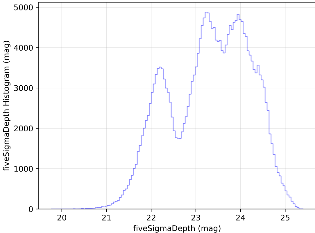
too_elab_r64_d3_gz_v3.4_10yrs Yr 1 all bands: fiveSigmaDepth Histogram
