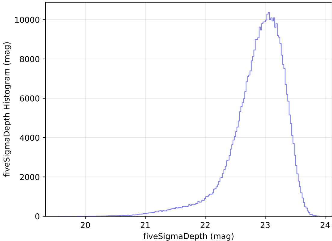
too_elab_r64_d3_gz_v3.4_10yrs WFD z band: fiveSigmaDepth Histogram
