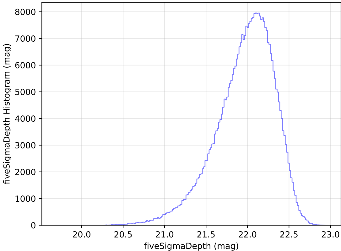
too_elab_r64_d3_gz_v3.4_10yrs WFD y band: fiveSigmaDepth Histogram
