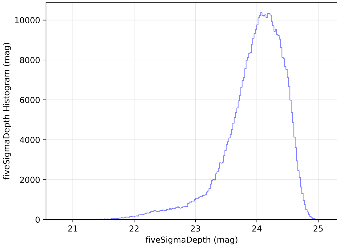
too_elab_r64_d3_gz_v3.4_10yrs WFD r band: fiveSigmaDepth Histogram
