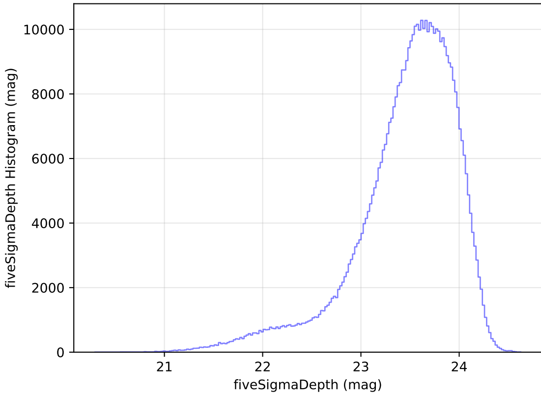
too_elab_r64_d3_gz_v3.4_10yrs WFD i band: fiveSigmaDepth Histogram
