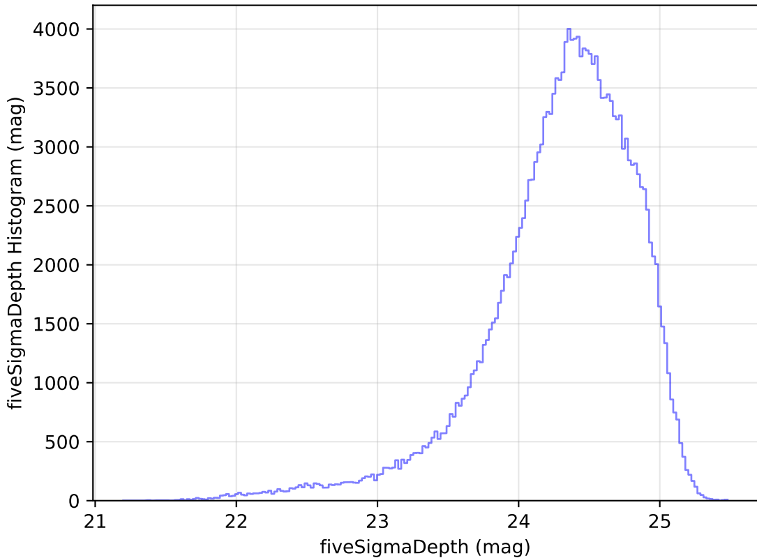
too_elab_r64_d3_gz_v3.4_10yrs WFD g band: fiveSigmaDepth Histogram
