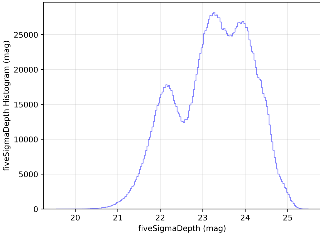
too_elab_r64_d3_gz_v3.4_10yrs WFD all bands: fiveSigmaDepth Histogram
