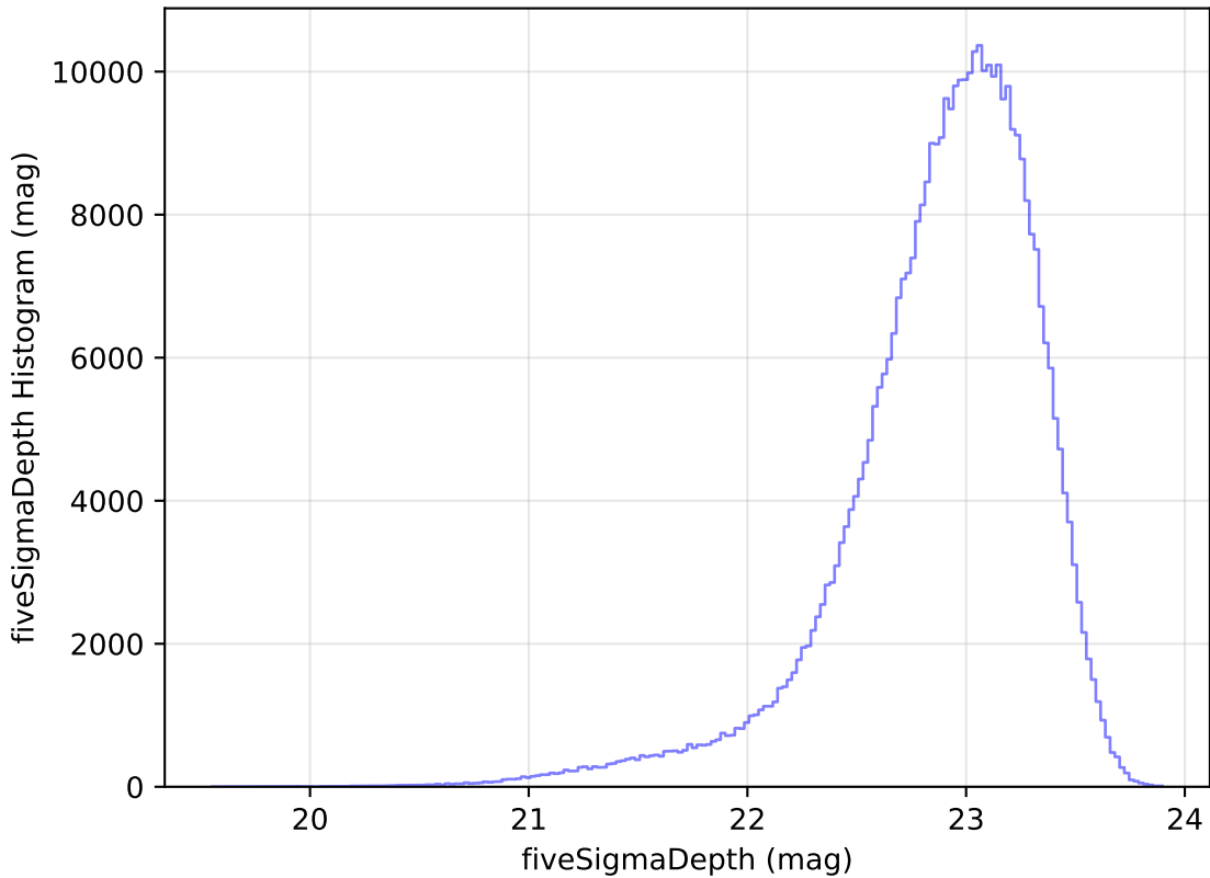
too_elab_r64_d3_gz_v3.4_10yrs All sky z band: fiveSigmaDepth Histogram
