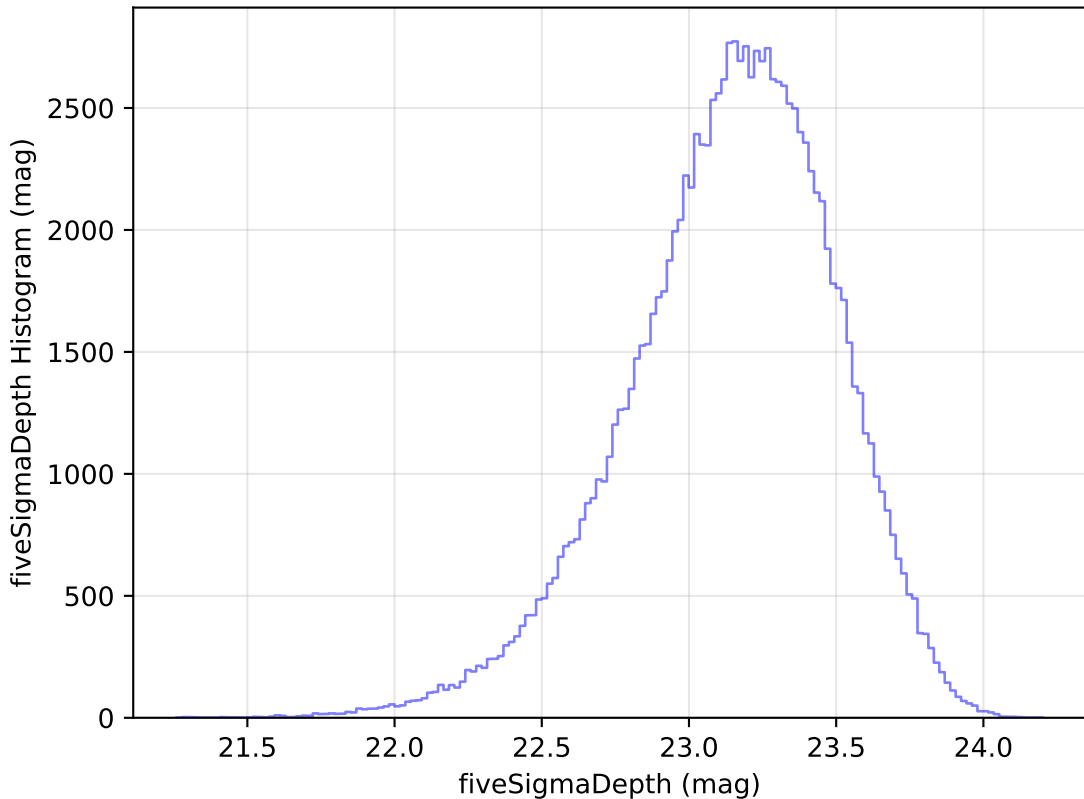
too_elab_r64_d3_gz_v3.4_10yrs All sky u band: fiveSigmaDepth Histogram
