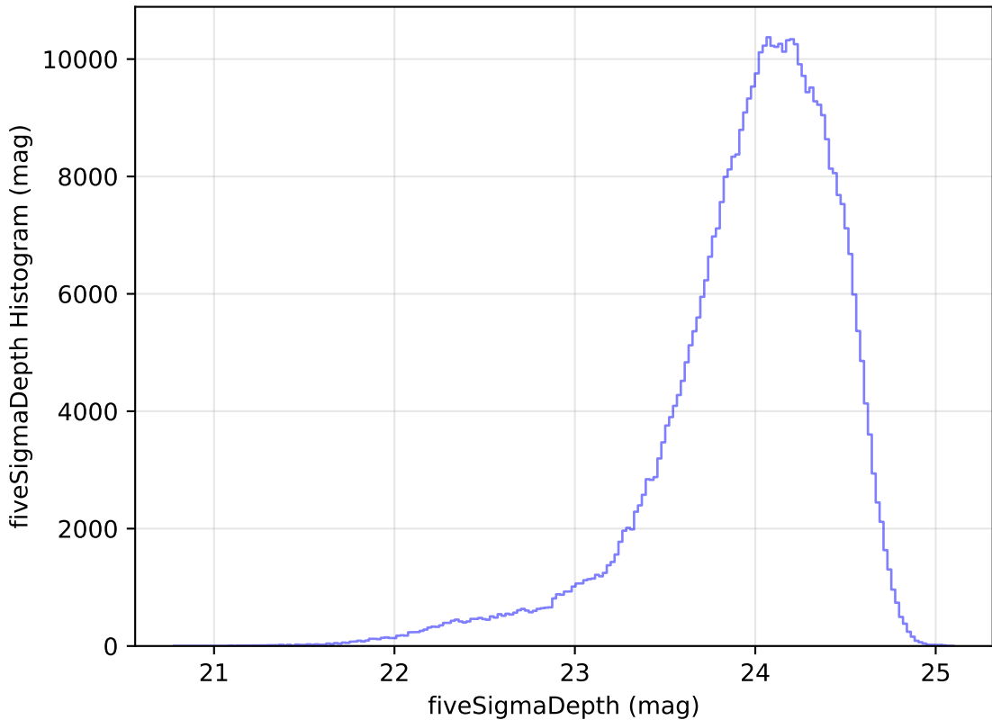
too_elab_r64_d3_gz_v3.4_10yrs All sky r band: fiveSigmaDepth Histogram
