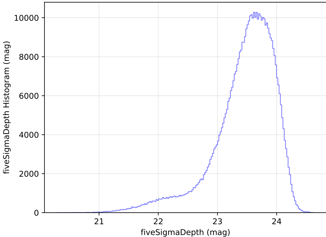
too_elab_r64_d3_gz_v3.4_10yrs All sky i band: fiveSigmaDepth Histogram
