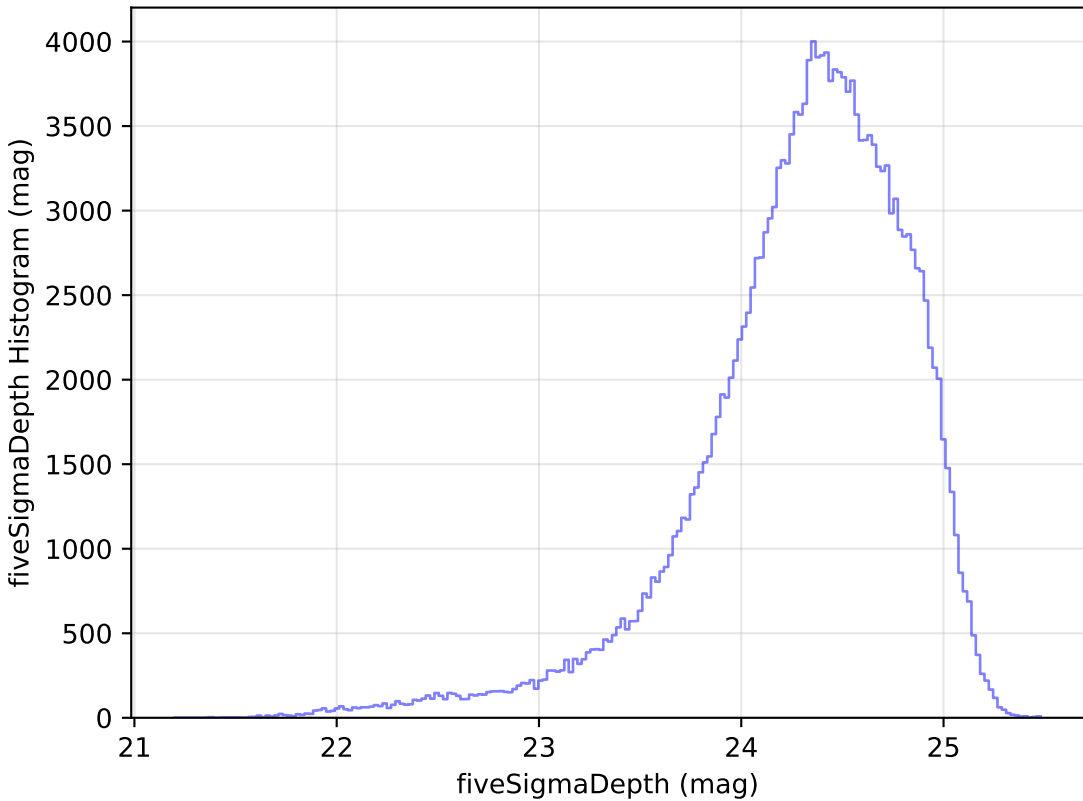
too_elab_r64_d3_gz_v3.4_10yrs All sky g band: fiveSigmaDepth Histogram
