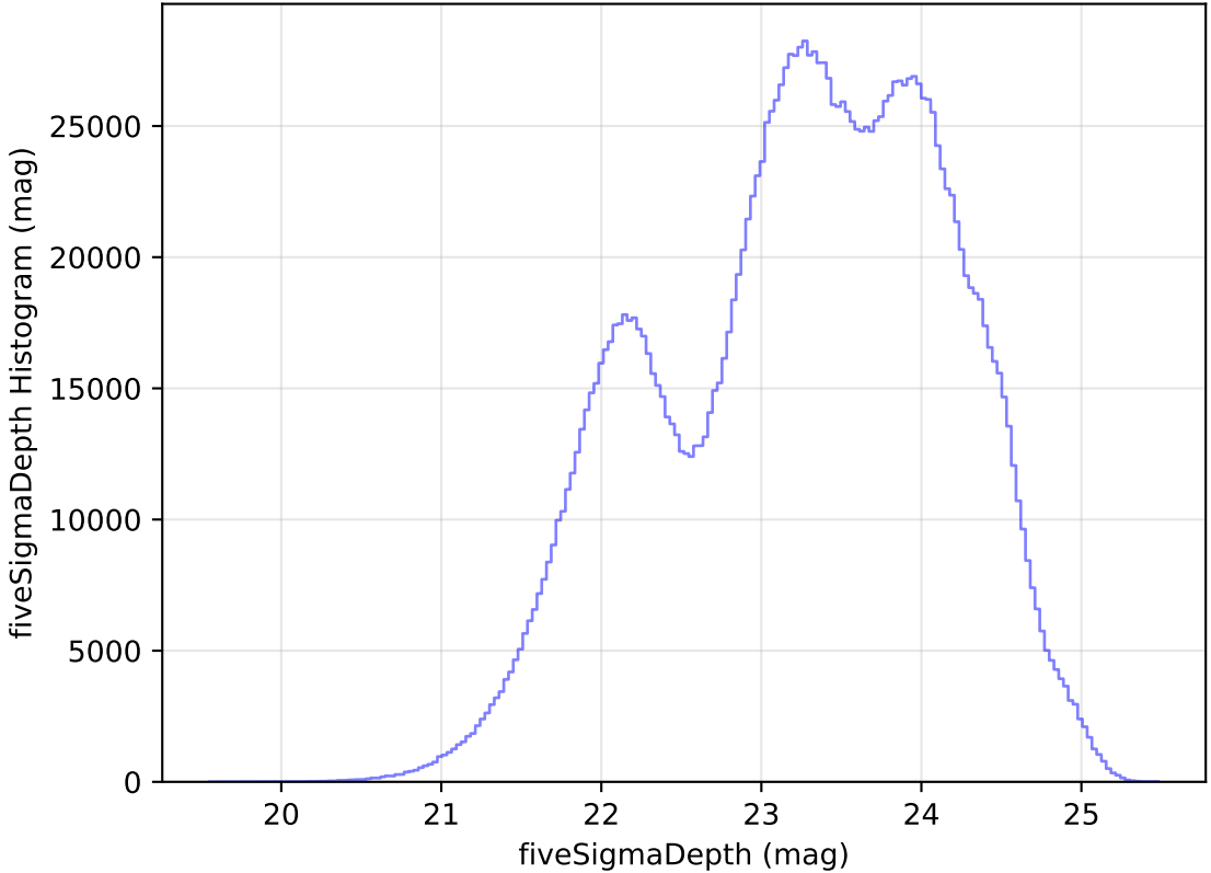
too_elab_r64_d3_gz_v3.4_10yrs All sky all bands: fiveSigmaDepth Histogram
