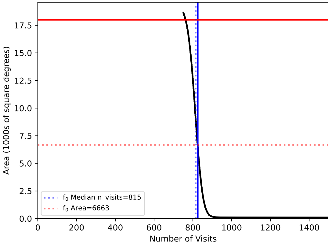
too_elab_r64_d3_gz_v3.4_10yrs WFD: f0
