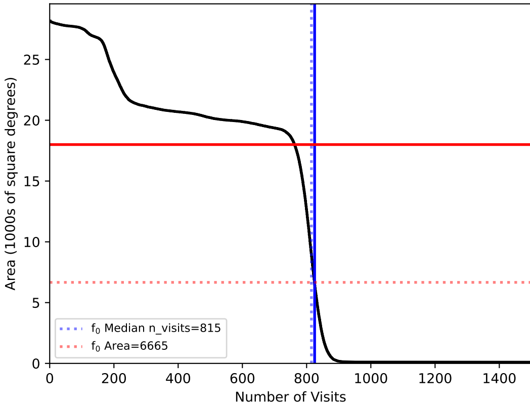
too_elab_r64_d3_gz_v3.4_10yrs All sky: f0
