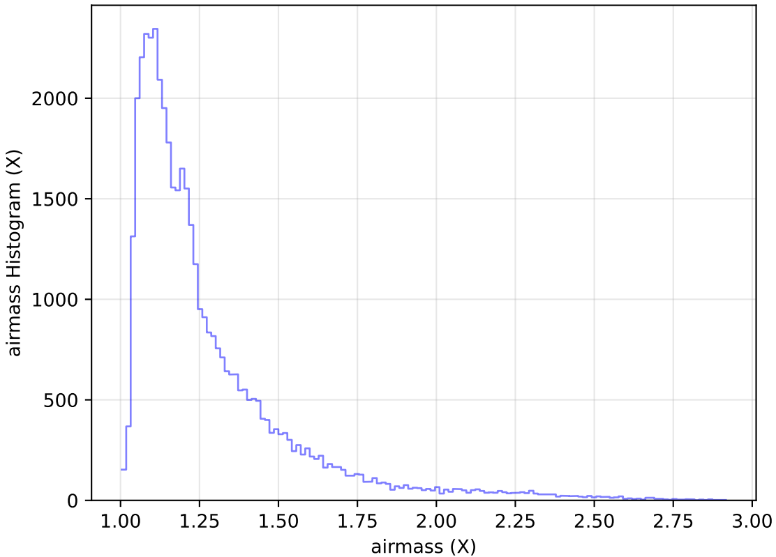
too_elab_r64_d3_gz_v3.4_10yrs Yr 1 z band: airmass Histogram
