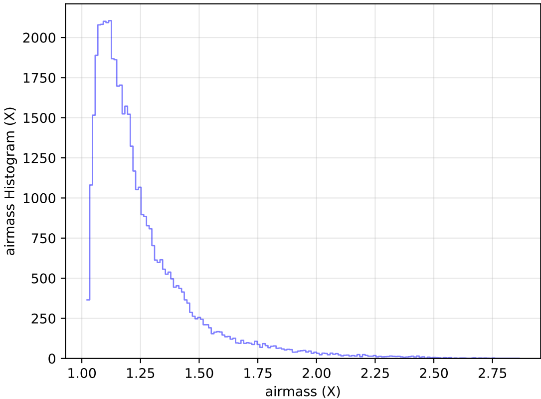
too_elab_r64_d3_gz_v3.4_10yrs Yr 1 y band: airmass Histogram
