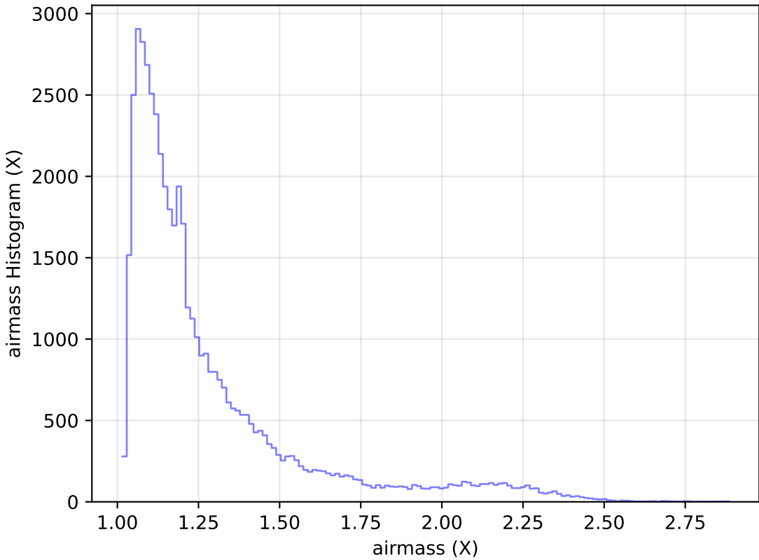
too_elab_r64_d3_gz_v3.4_10yrs Yr 1 r band: airmass Histogram
