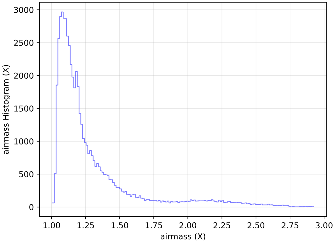
too_elab_r64_d3_gz_v3.4_10yrs Yr 1 i band: airmass Histogram
