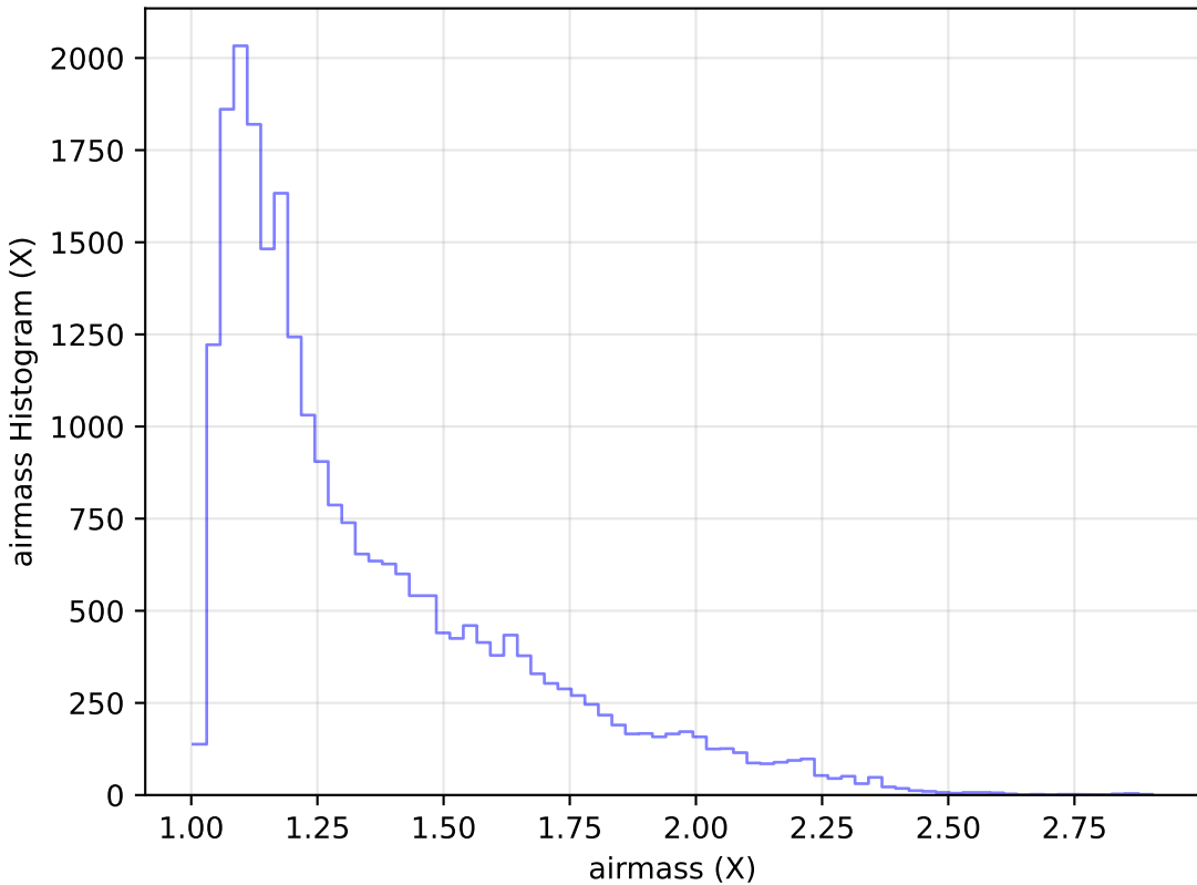
too_elab_r64_d3_gz_v3.4_10yrs Yr 1 g band: airmass Histogram
