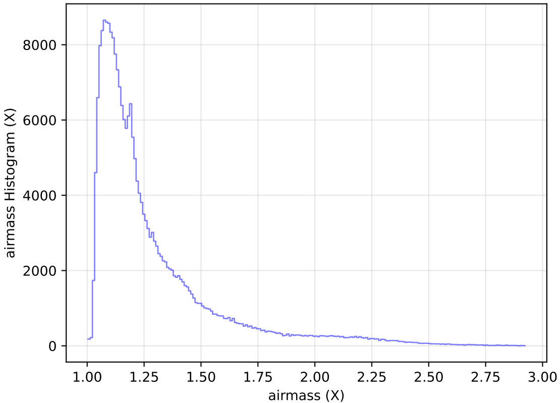
too_elab_r64_d3_gz_v3.4_10yrs Yr 1 all bands: airmass Histogram
