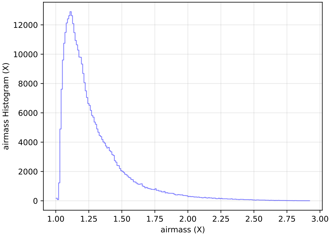
too_elab_r64_d3_gz_v3.4_10yrs WFD y band: airmass Histogram
