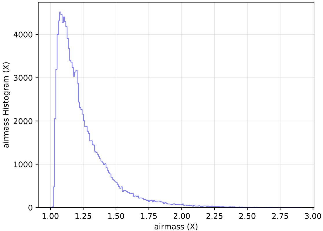
too_elab_r64_d3_gz_v3.4_10yrs WFD u band: airmass Histogram
